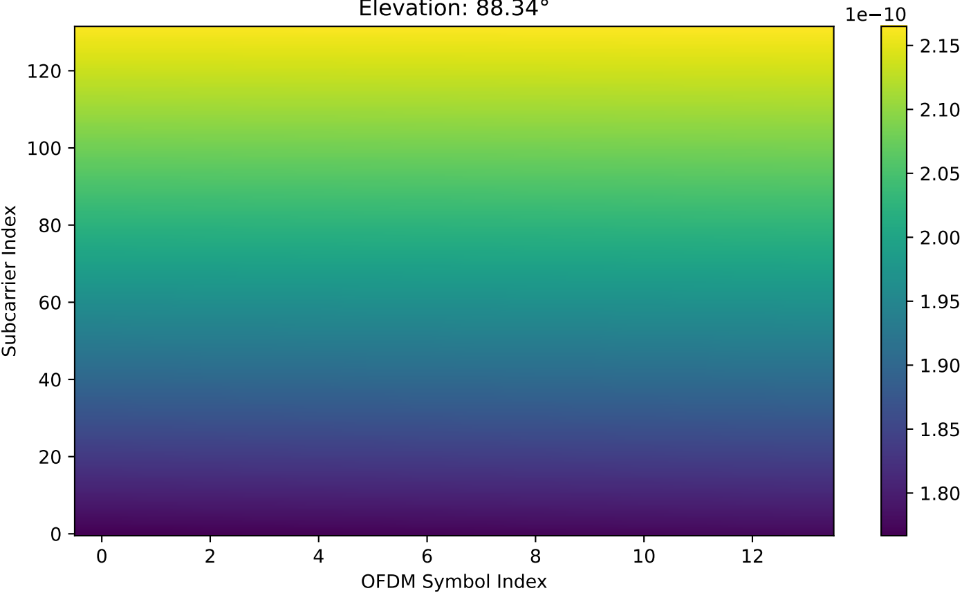
Precompensated Doppler: Real Part of Channel 0 (SUR) Elevation: 88.34°
