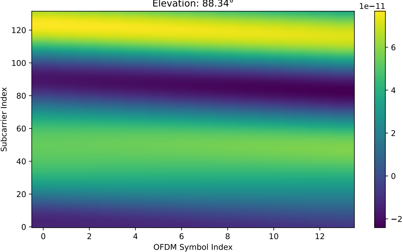
Precompensated Doppler: Real Part of Channel 0 (DUR) Elevation: 88.34°
