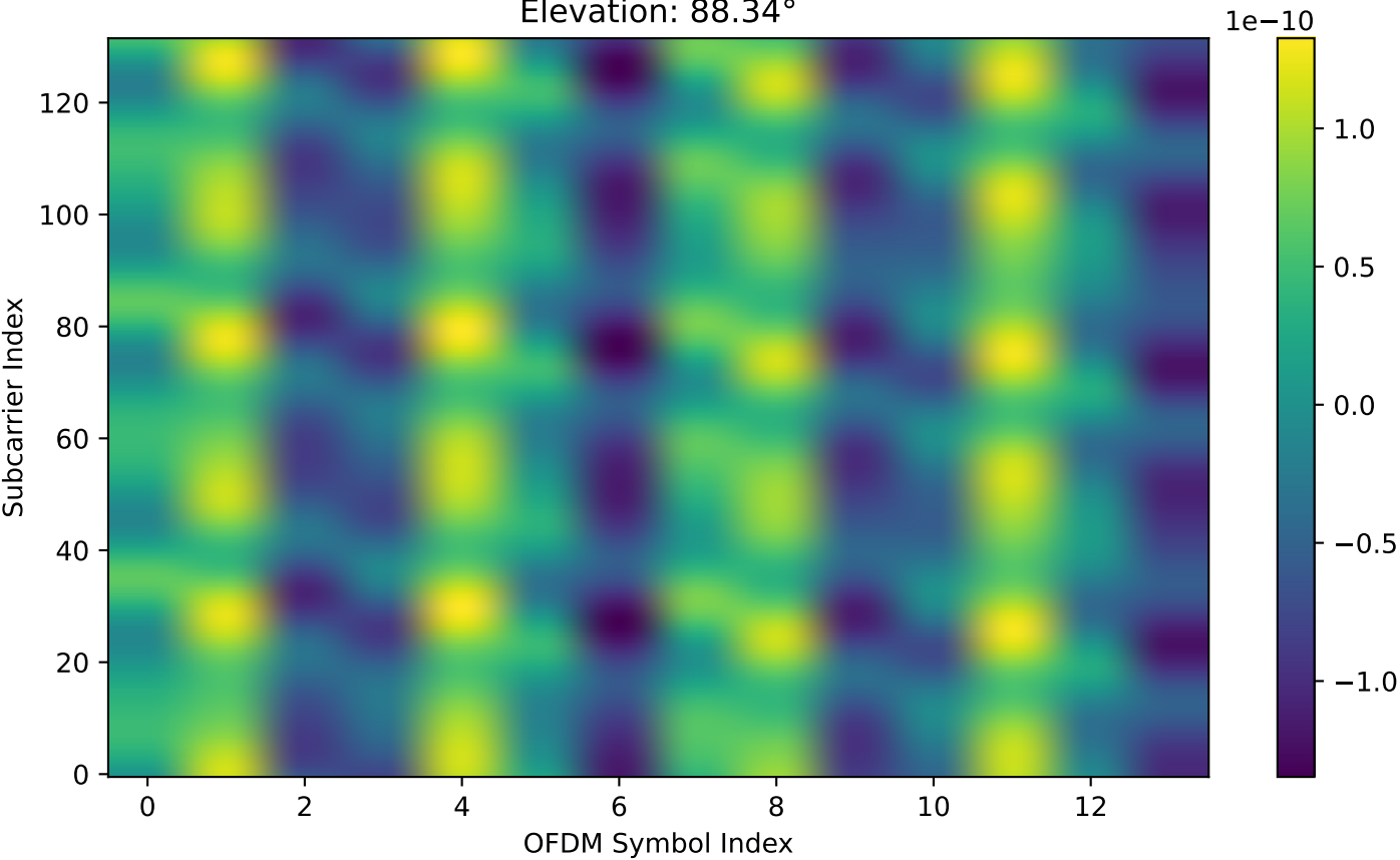
Full Doppler: Real Part of Channel 0 (DUR) Elevation: 88.34°
