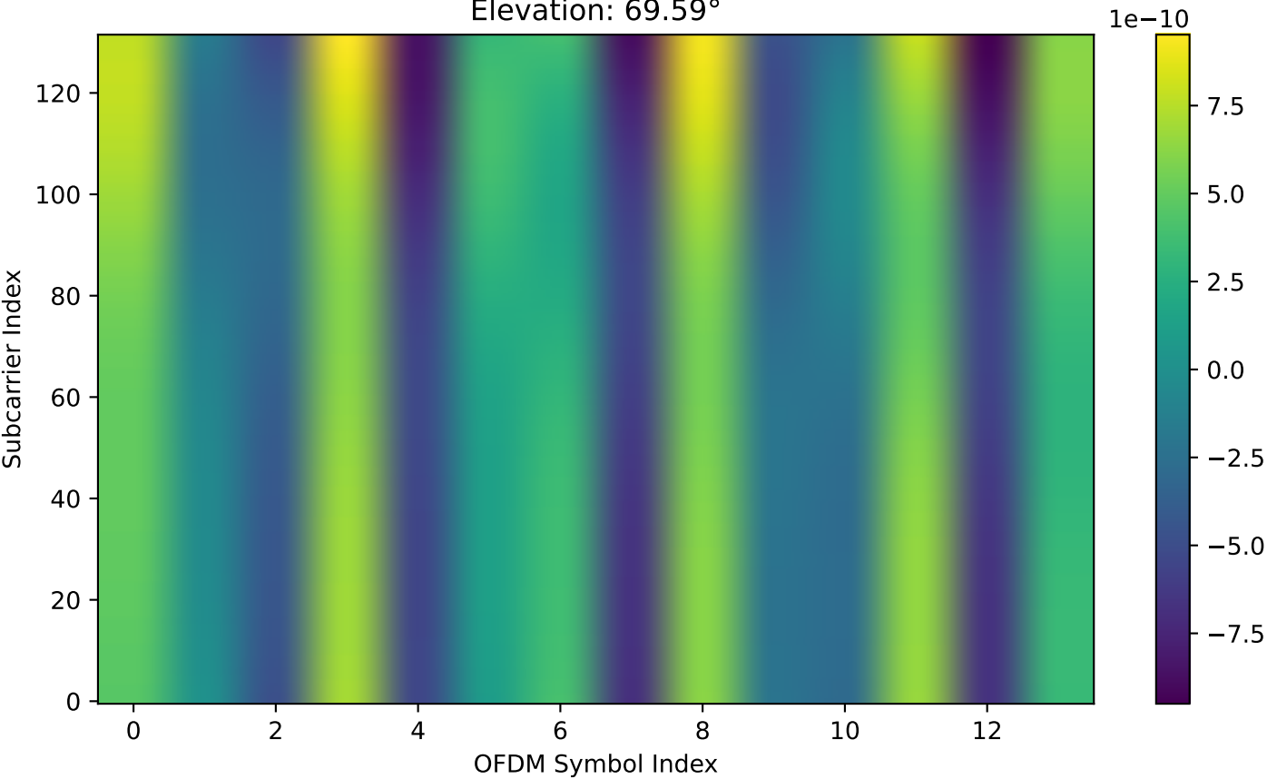
Original Perfect Channel (Full Doppler): Real Part of Channel 0 (DUR) Elevation: 69.59^\circ
