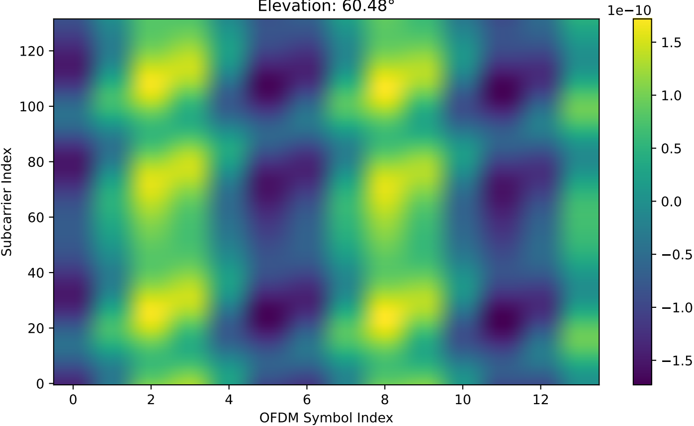
Original Perfect Channel (Full Doppler): Real Part of Channel 0 (SUR) Elevation: 60.48°
