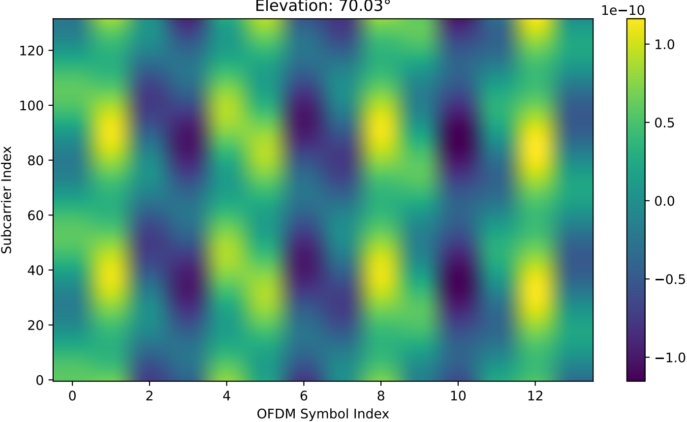
Original Perfect Channel (Full Doppler): Real Part of Channel 0 (SUR) Elevation: 70.03^\circ
