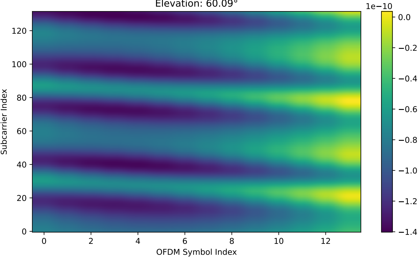
Original Perfect Channel (Full Doppler): Real Part of Channel 0 (SUR) Elevation: 60.09°
