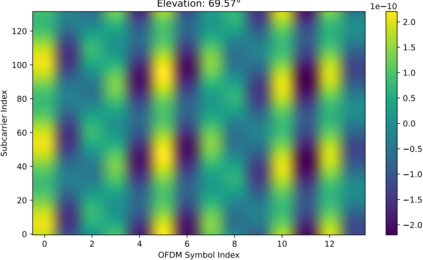
Original Perfect Channel (Full Doppler): Real Part of Channel 0 (SUR) Elevation: 69.57^\circ
