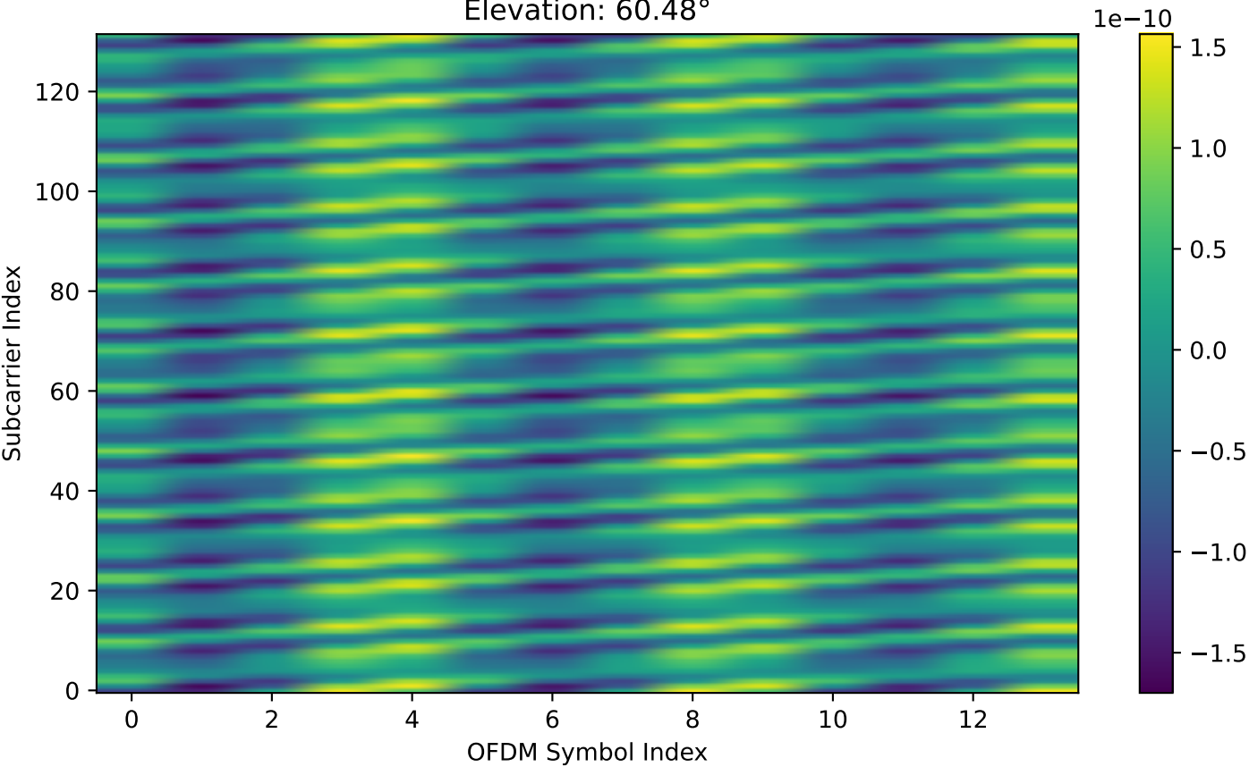
Original Perfect Channel (Full Doppler): Real Part of Channel 0 (SUR) Elevation: 60.48^\circ
