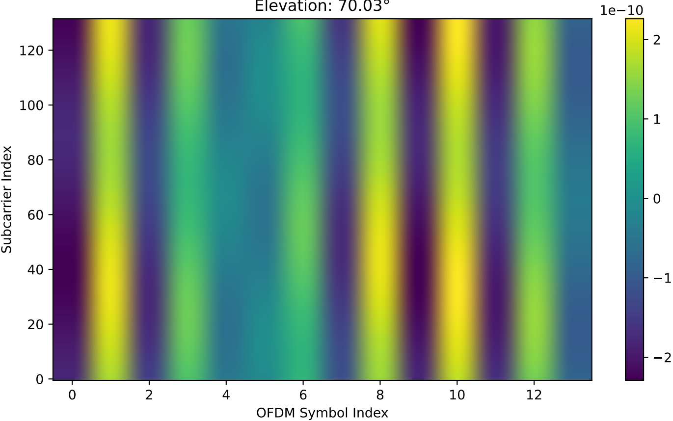
Original Perfect Channel (Full Doppler): Real Part of Channel 0 (SUR) Elevation: 70.03^\circ
