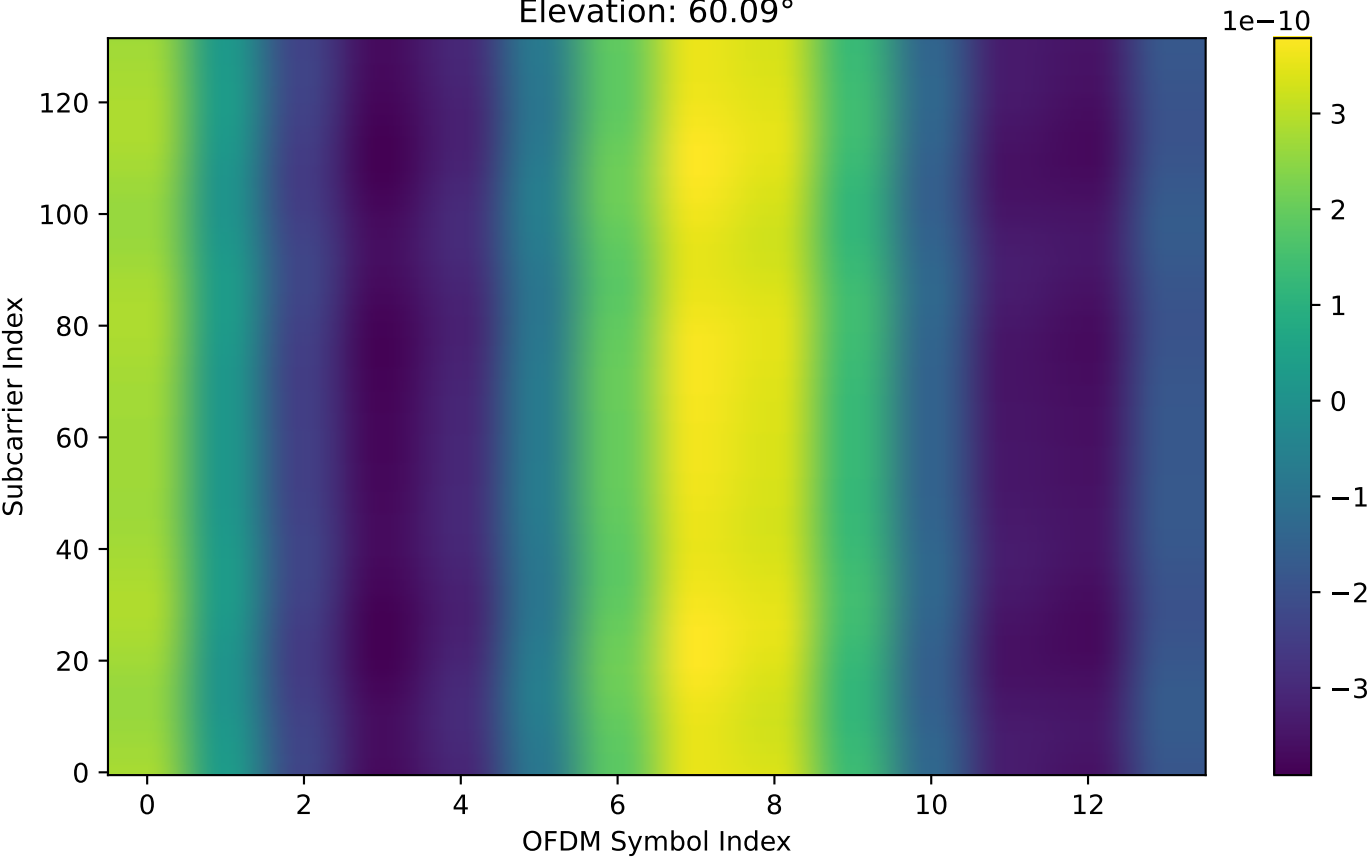
Original Perfect Channel (Full Doppler): Real Part of Channel 0 (SUR) Elevation: 60.09°
