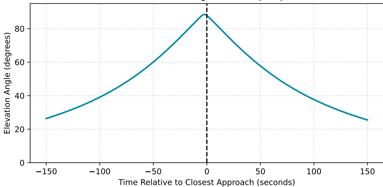
Satellite Elevation Angle from UE perspective
