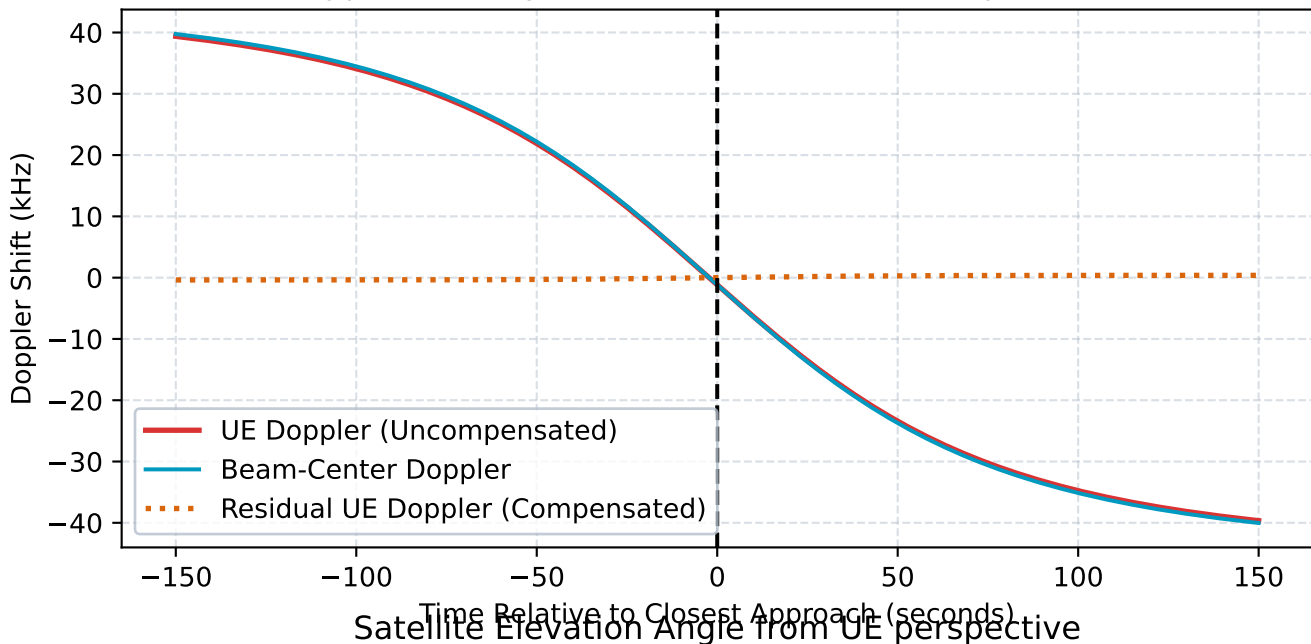
Doppler Shift Dynamics (S-Curve & Pre-compensation)
