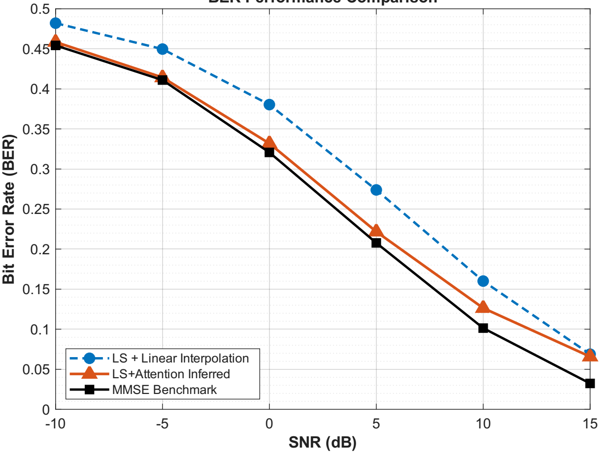
BER Performance Comparison
