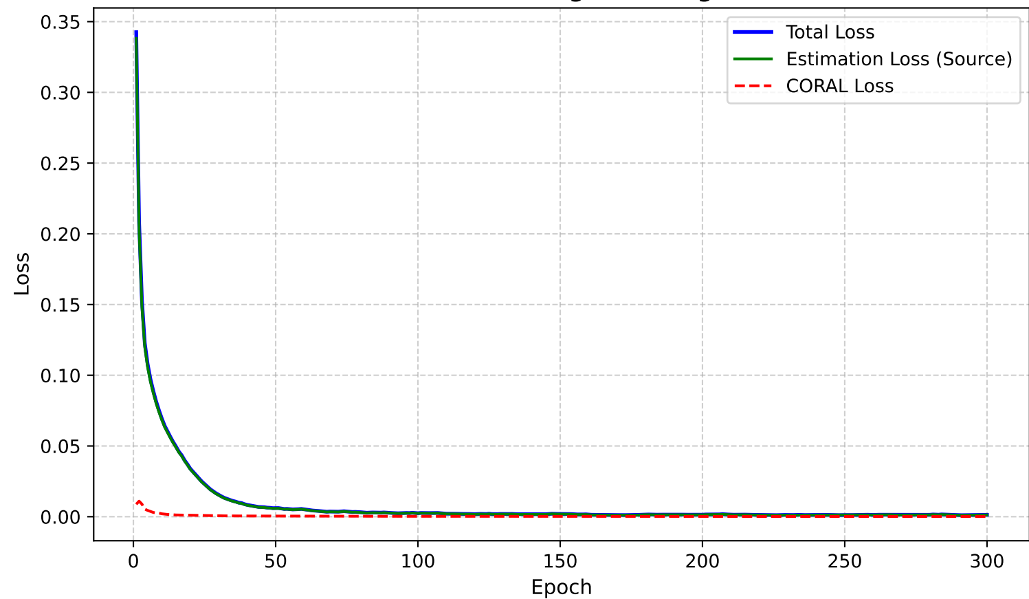
HA02 CORAL Training Loss Progression
