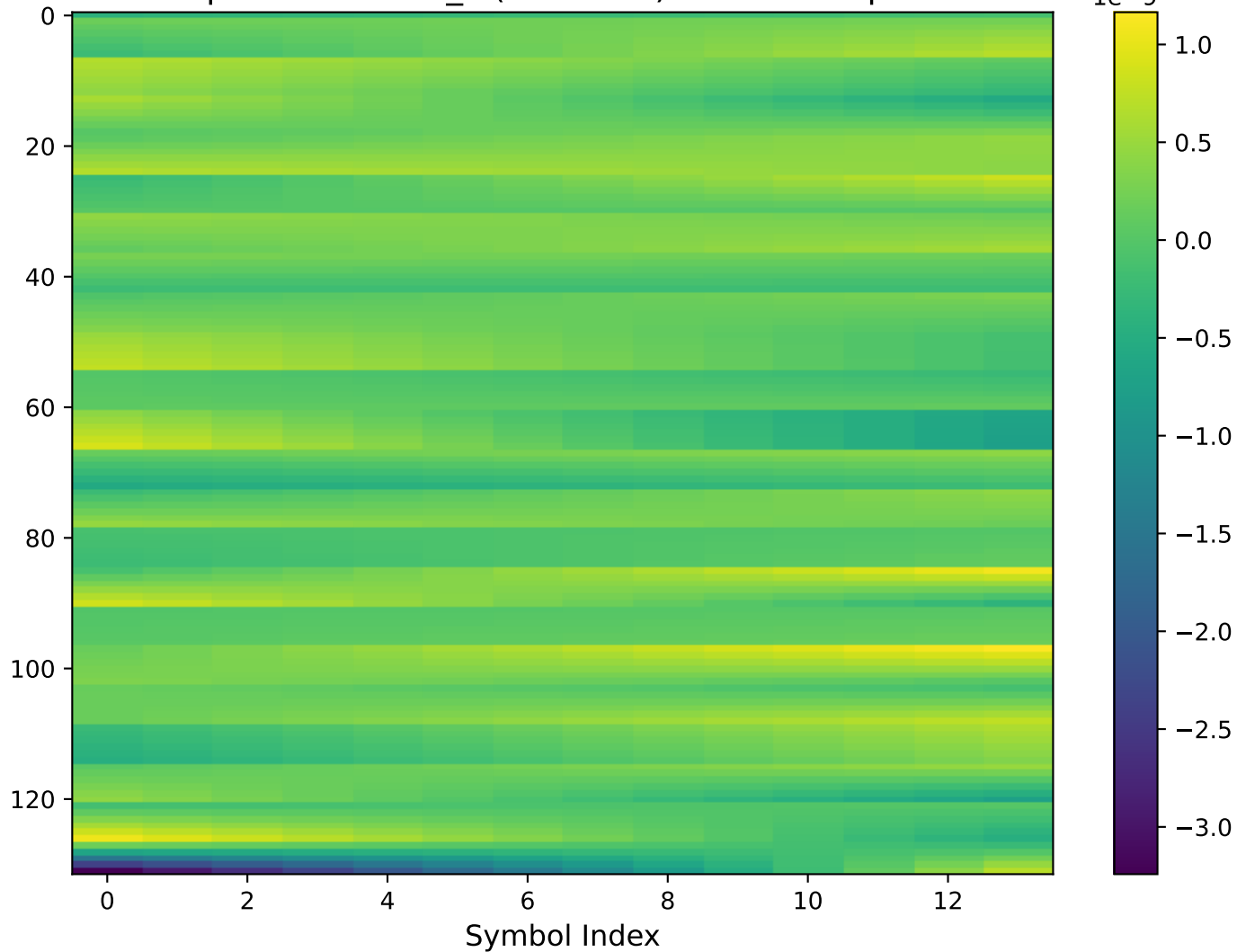
Input Channel H li (Real Part) - Train Sample 1
