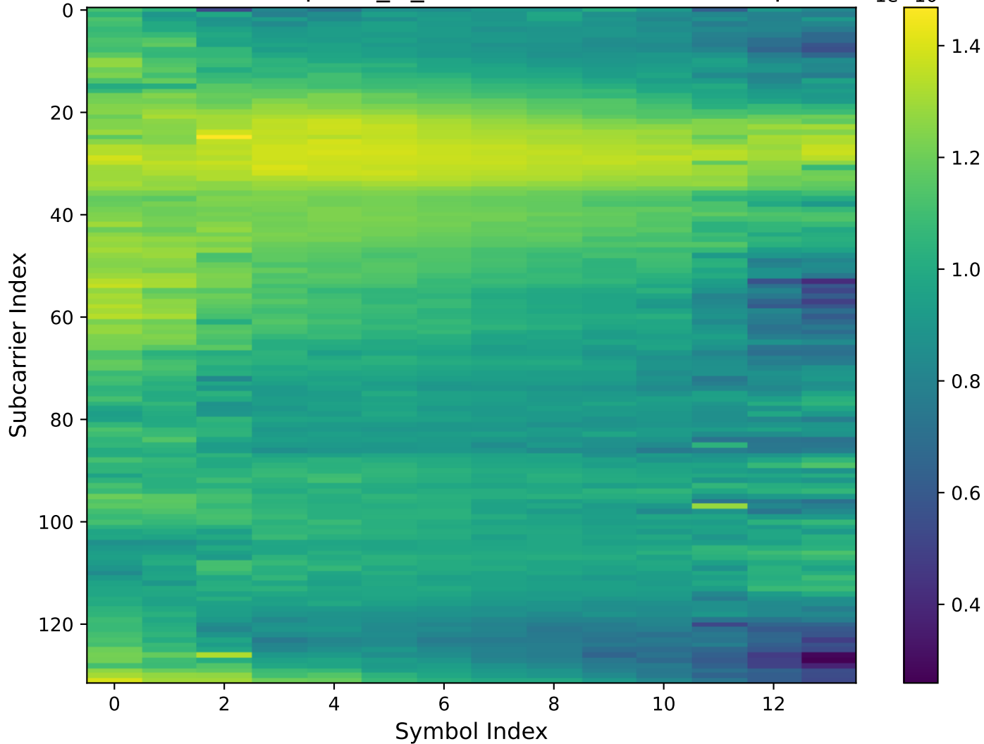
CNN Model Output H_ls_cnn (Real Part) - Train Sample 1
