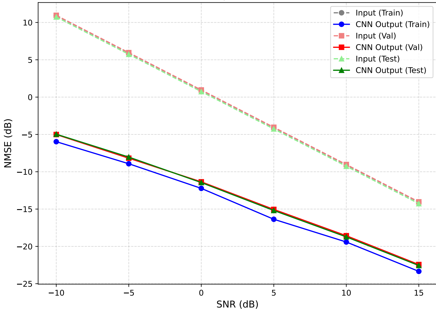
NMSE (dB) Comparison over SNR (LI)
