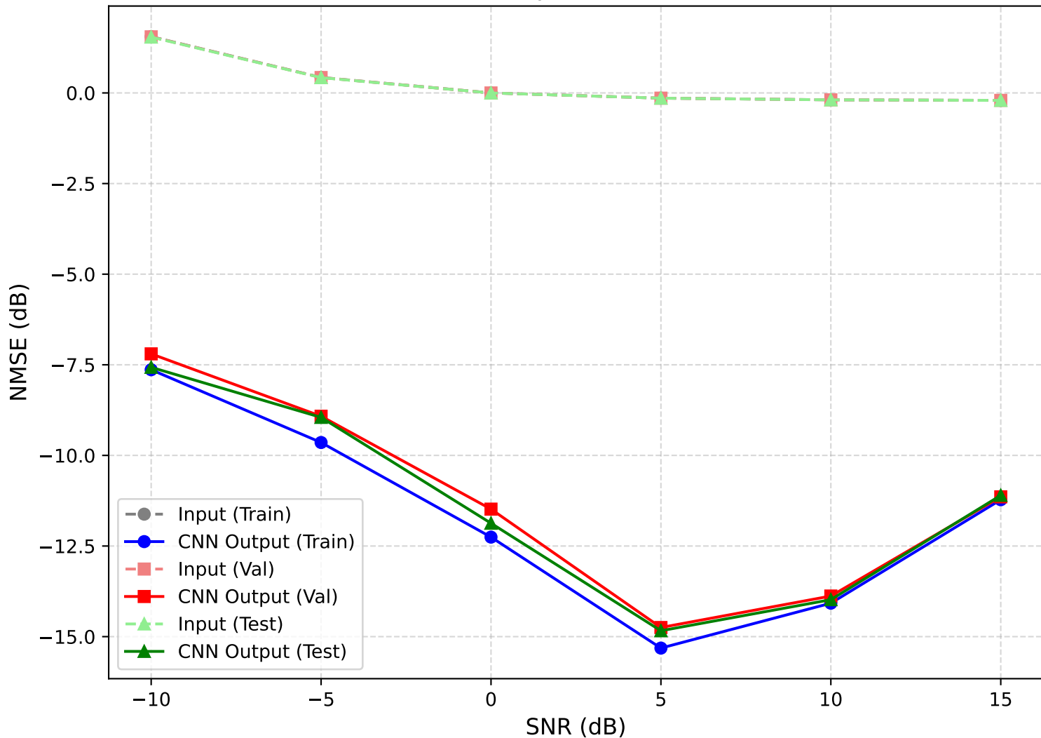
NMSE (dB) Comparison over SNR (LS)
