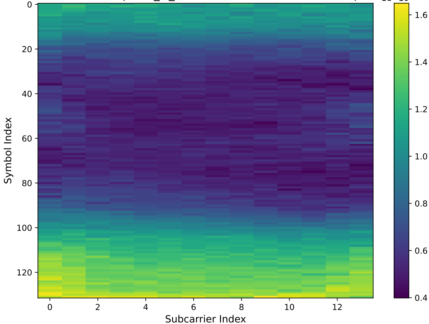
HA02 Model Output H_Is_attention (Real Part) - Test Sample 1_{1e-10}
