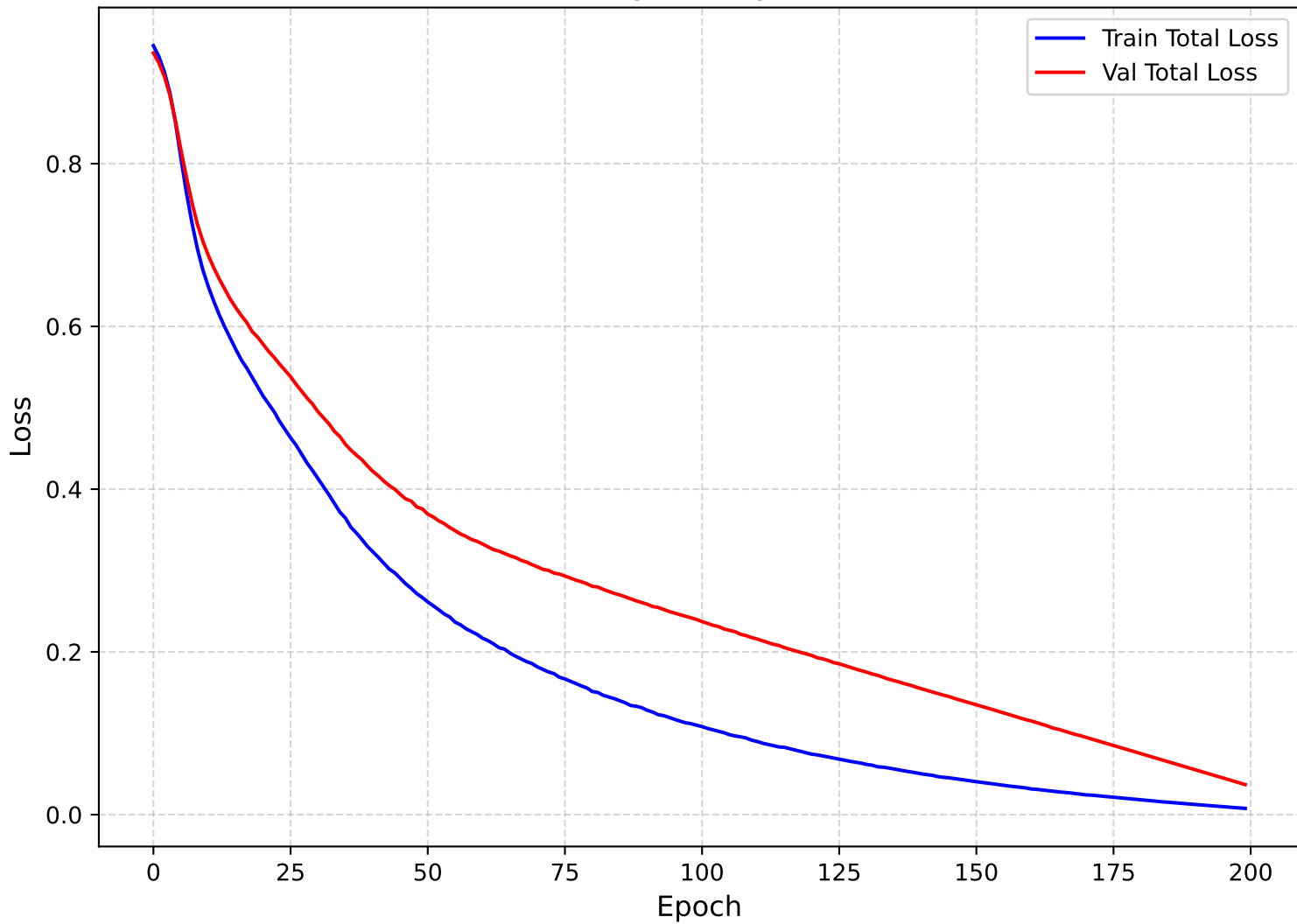
Training History - Loss
