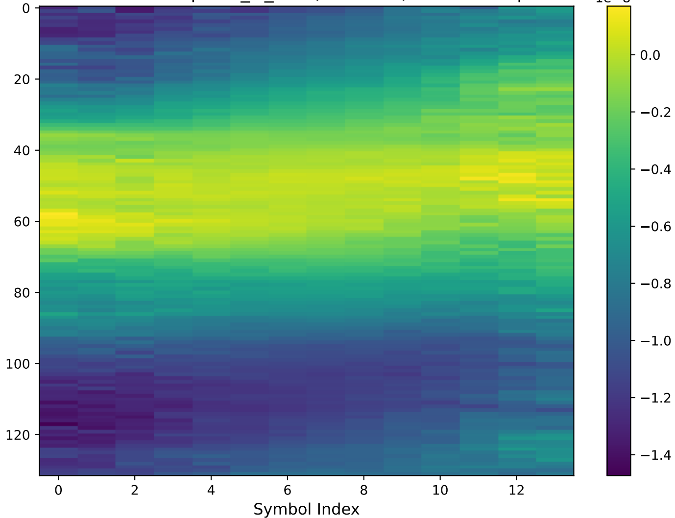
CNN Model Output H_ls_cnn (Real Part) - Train Sample 1
