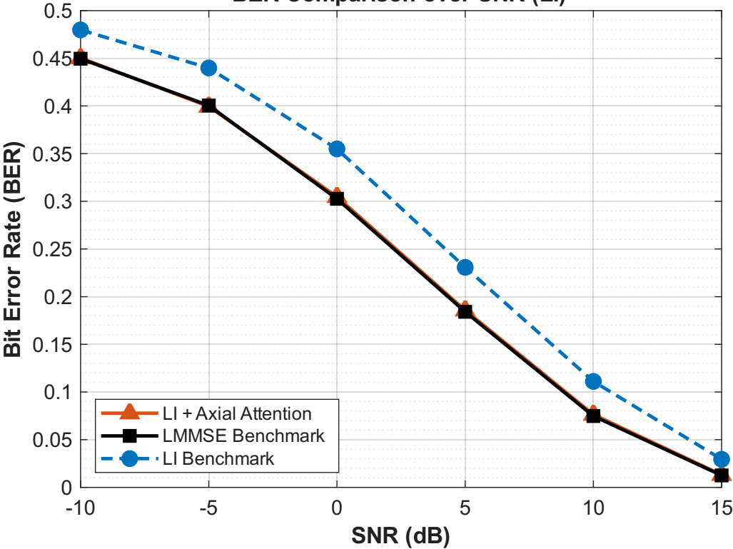
BER Comparison over SNR (LI)
