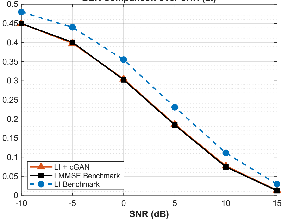
BER Comparison over SNR (LI)
