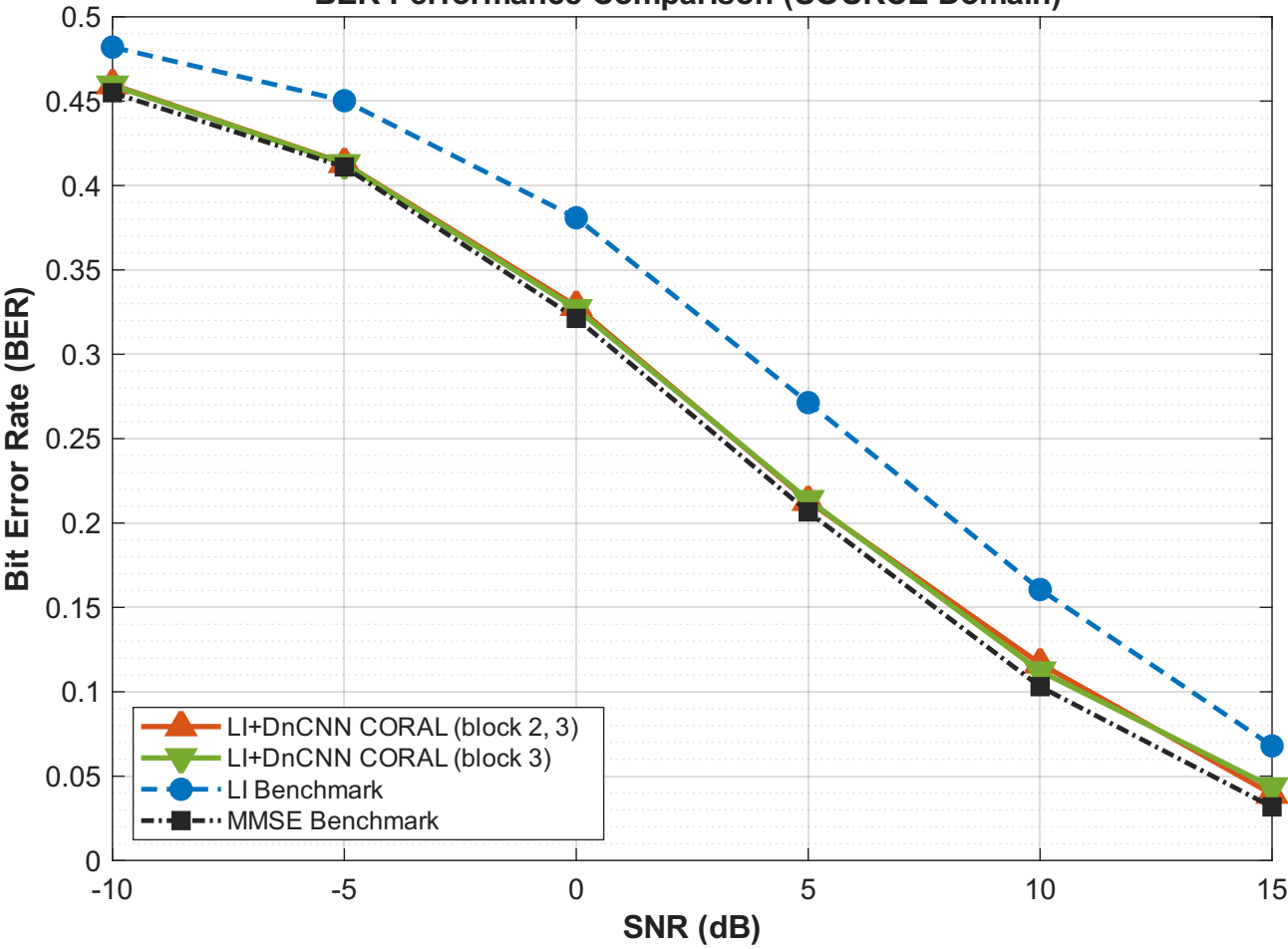
BER Performance Comparison (SOURCE Domain)
