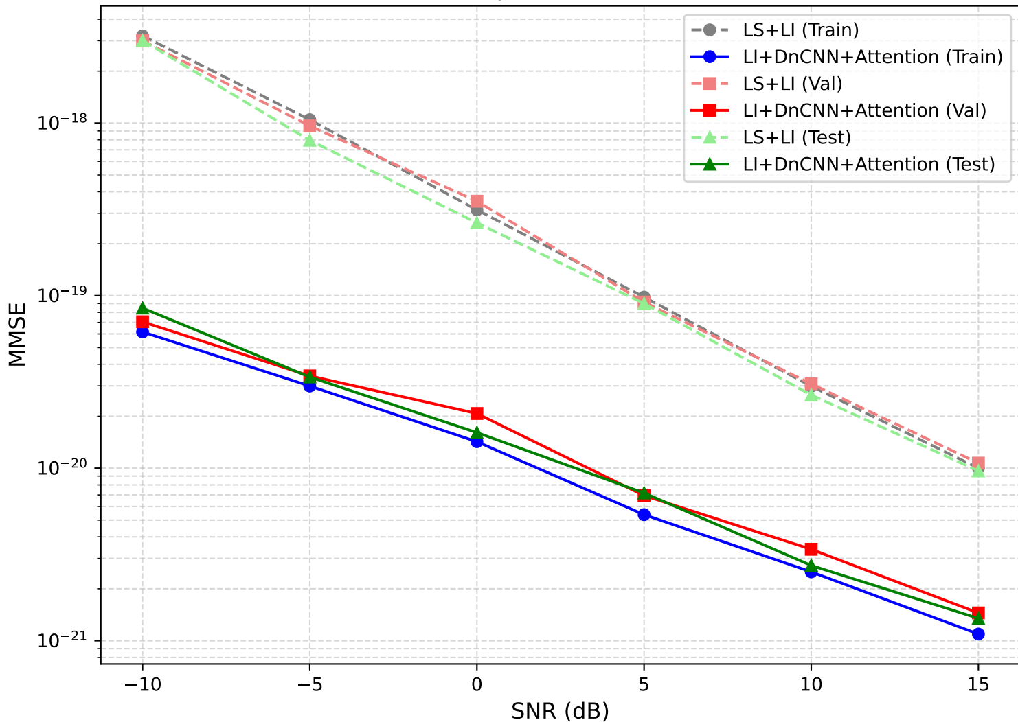
MMSE Comparison over SNR (LI)
