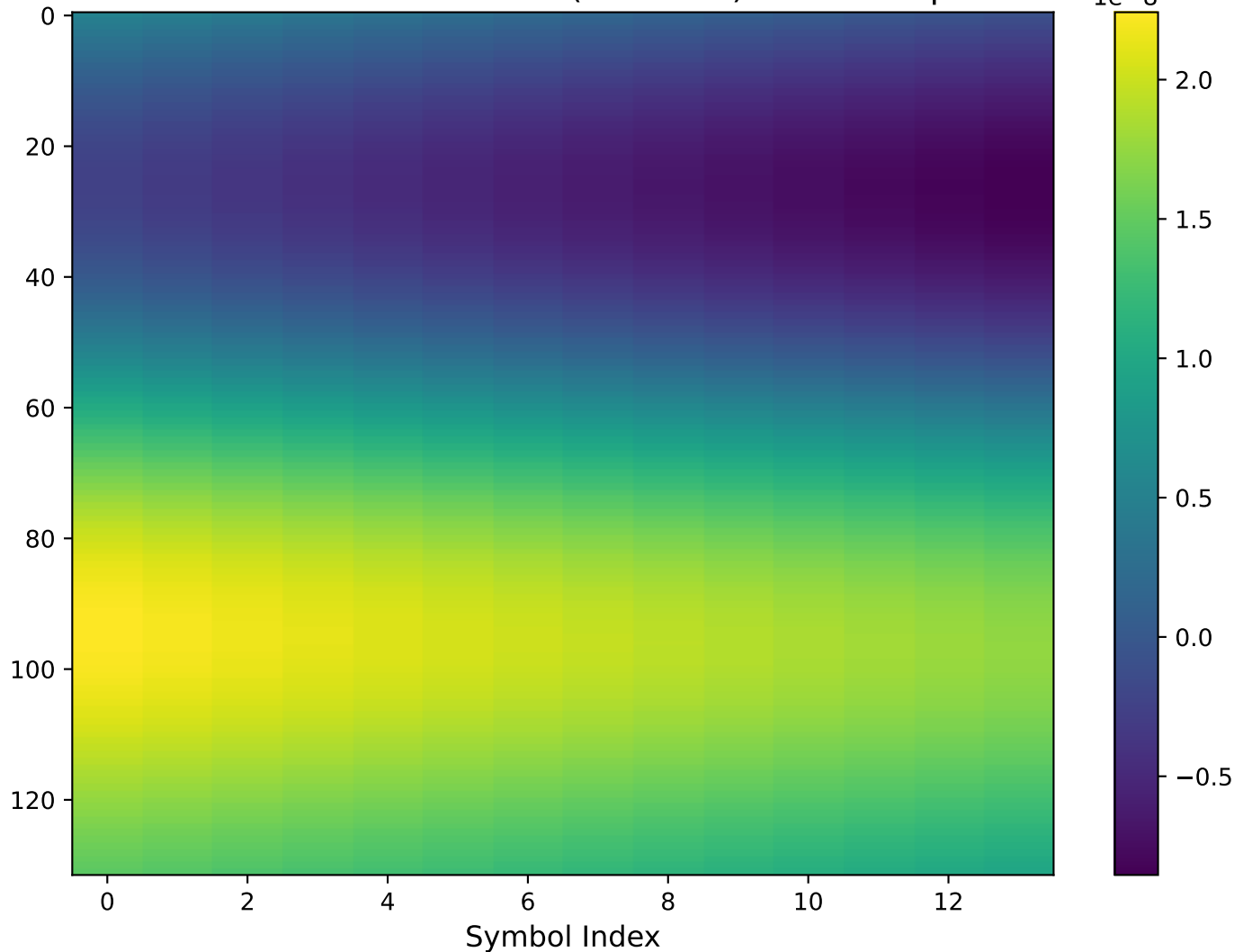
Perfect Reference Channel (Real Part) - Test Sample 1
