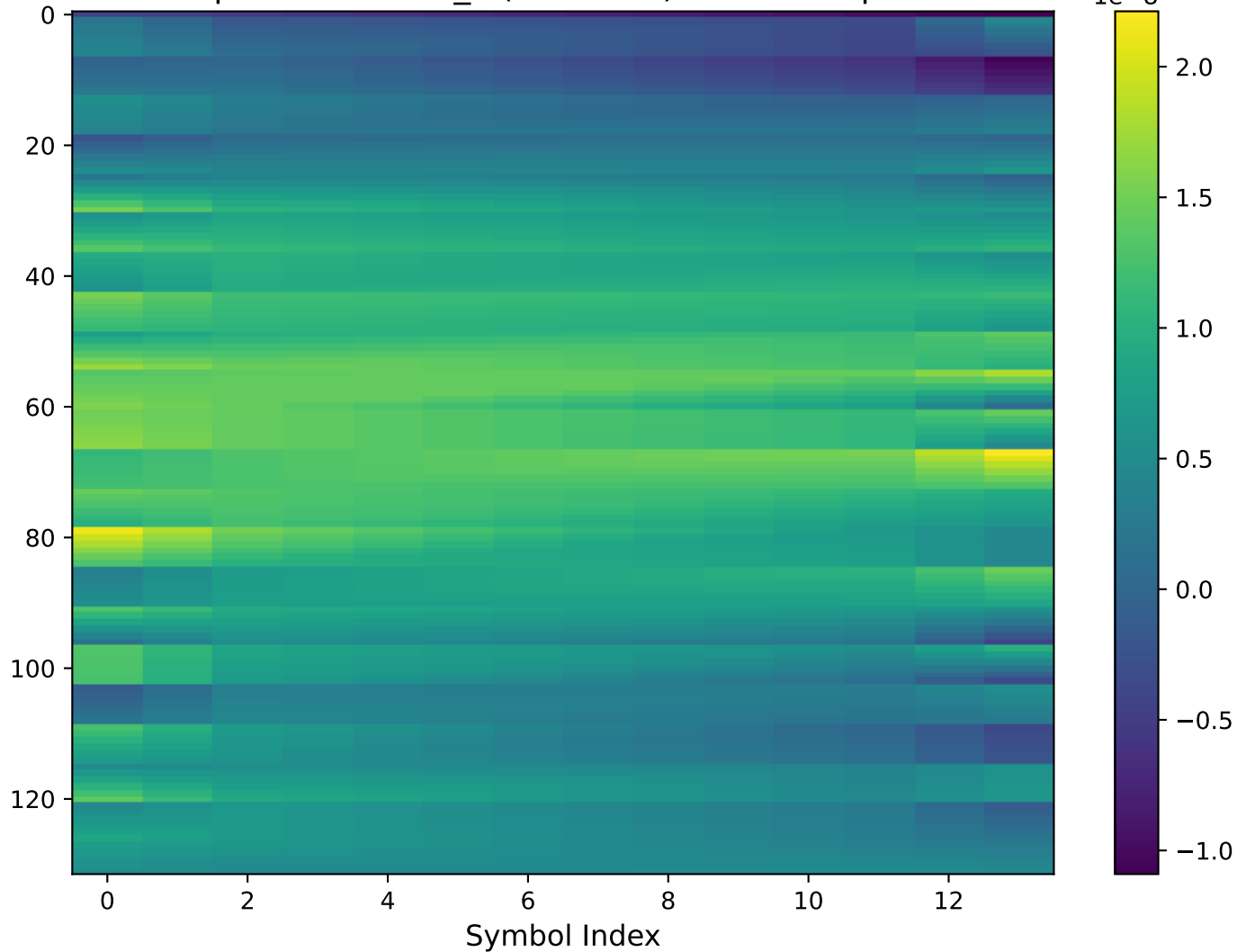
Input Channel H_li (Real Part) - Test Sample 1
