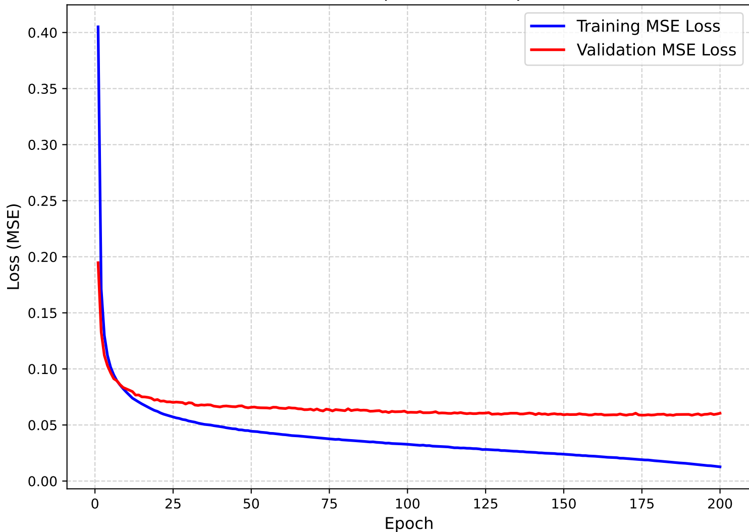
MSE Loss Component over Epochs
