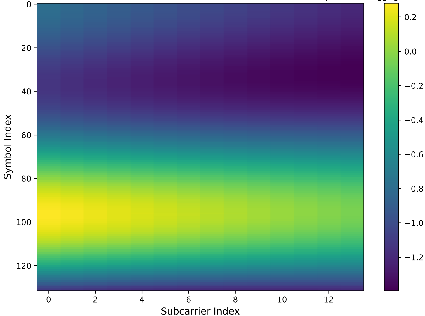
Perfect Reference Channel (Real Part) - Train Sample 1
