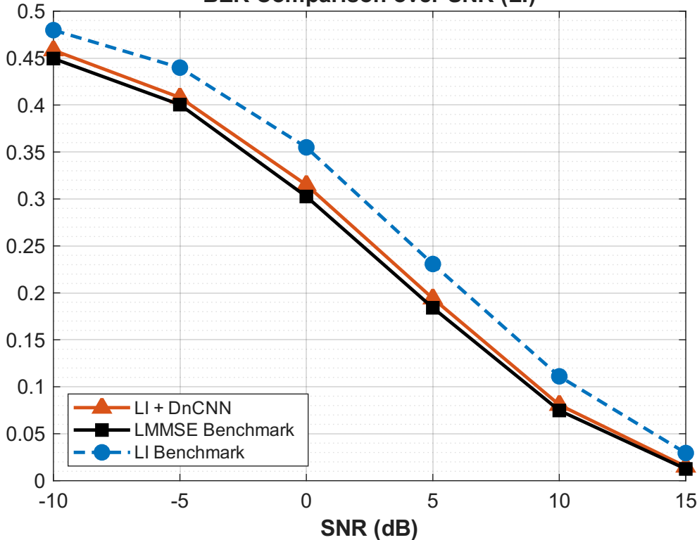
BER Comparison over SNR (LI)
