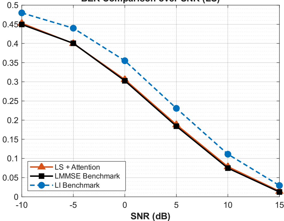
BER Comparison over SNR (LS)
