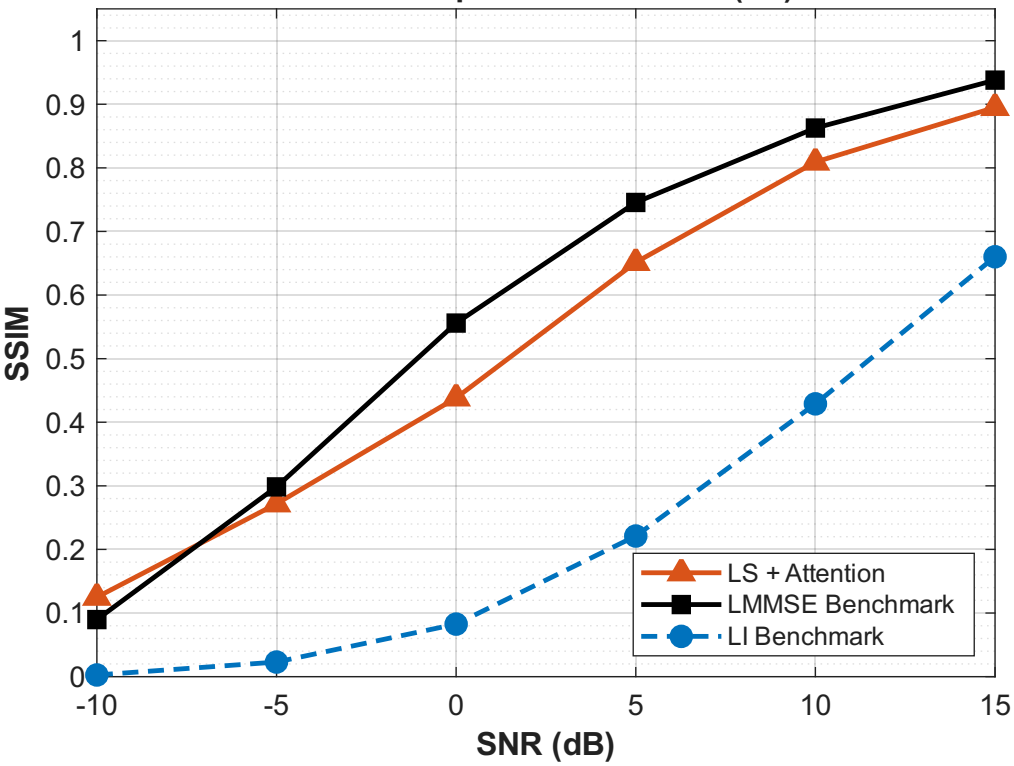
SSIM Comparison over SNR (LS)
