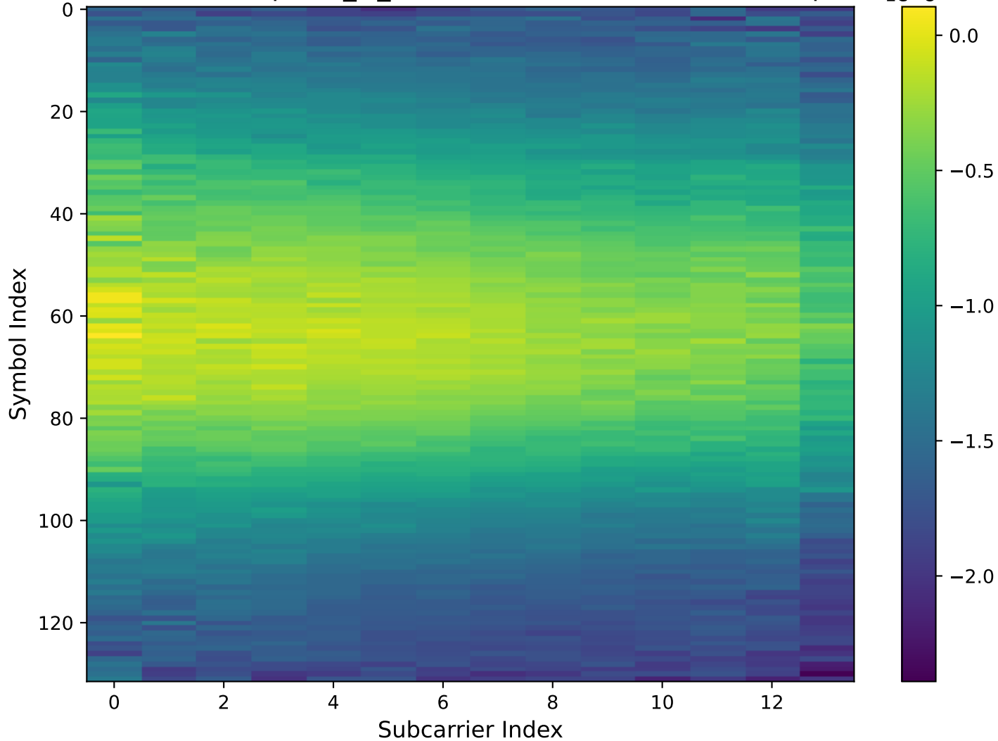
HA02 cGAN Output H_Is_attention (Real Part) - Train Sample 1 1e-8
