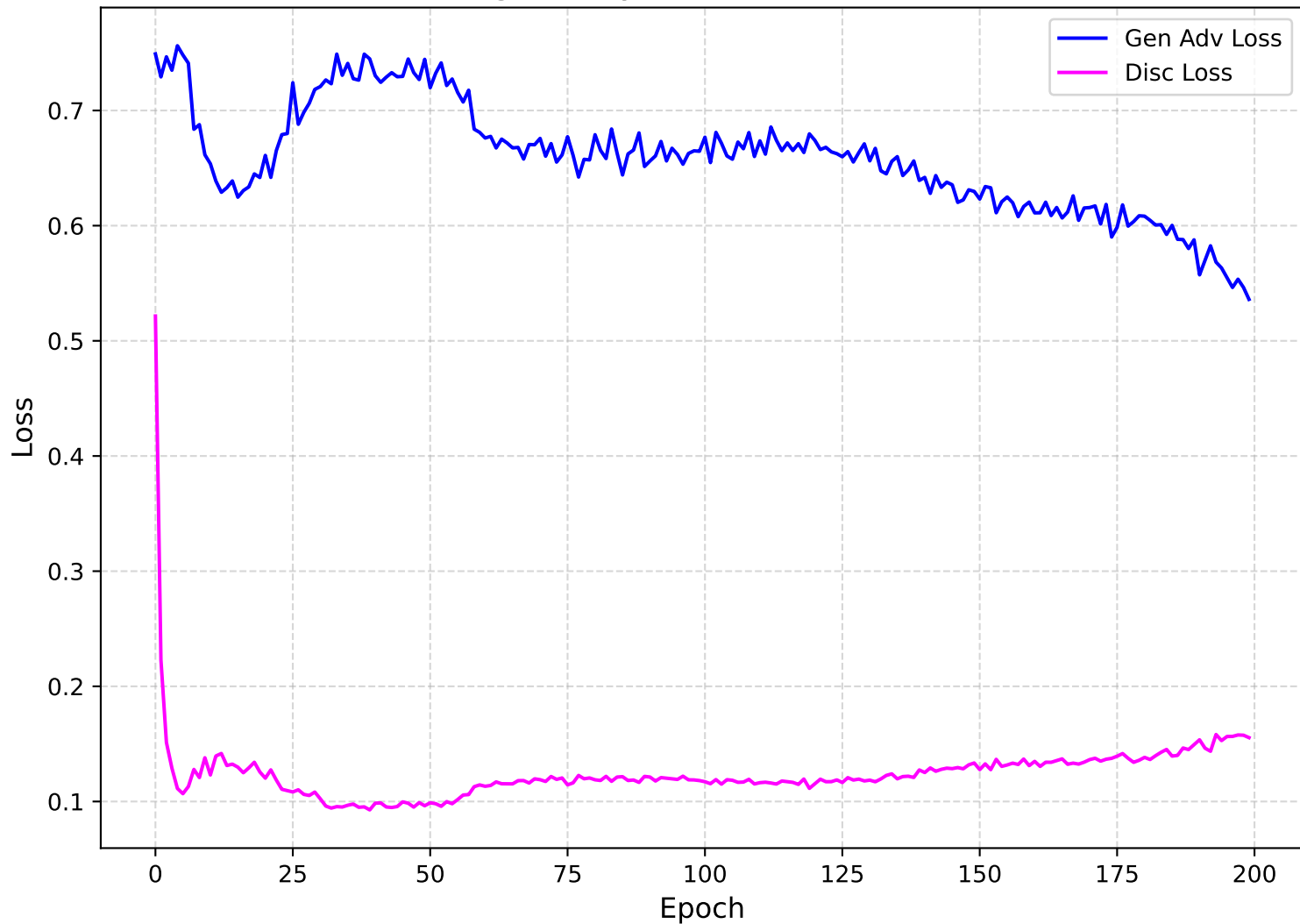
Training History - GAN Adversarial Loss
