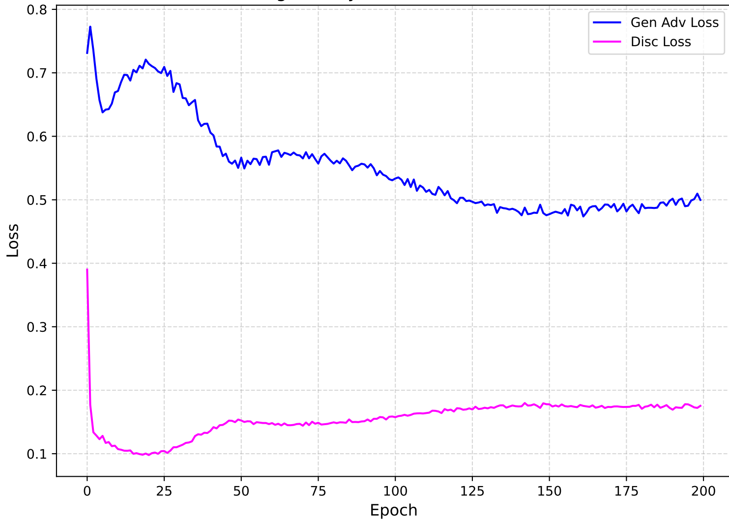
Training History - GAN Adversarial Loss
