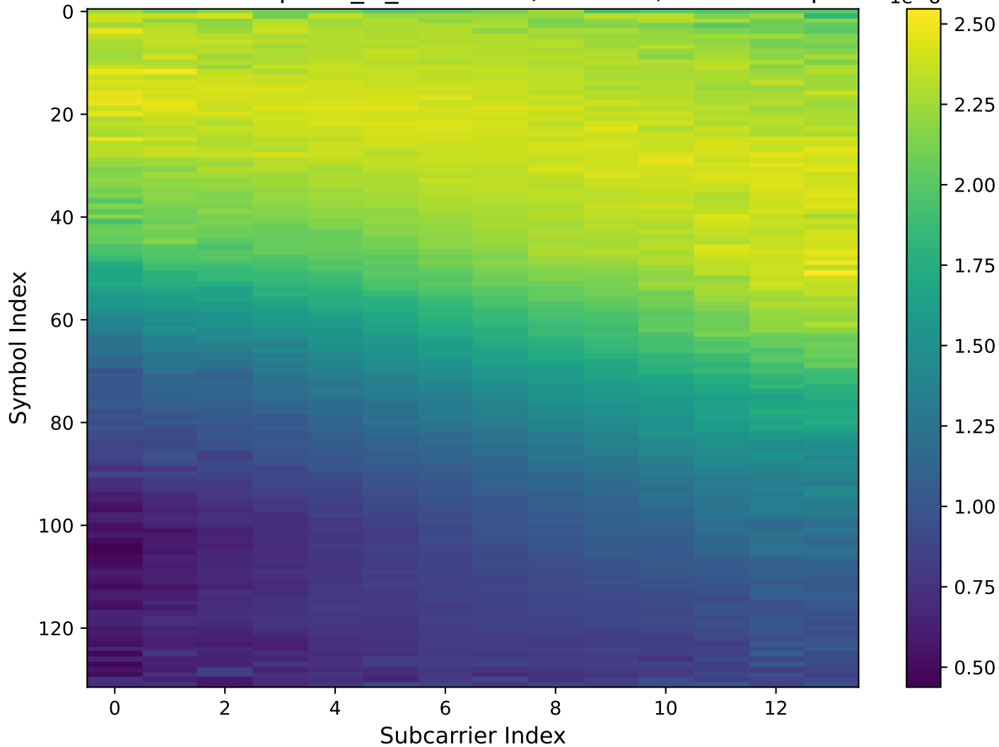
HA02 cGAN Output H_Is_attention (Real Part) - Test Sample 1 1e-8
