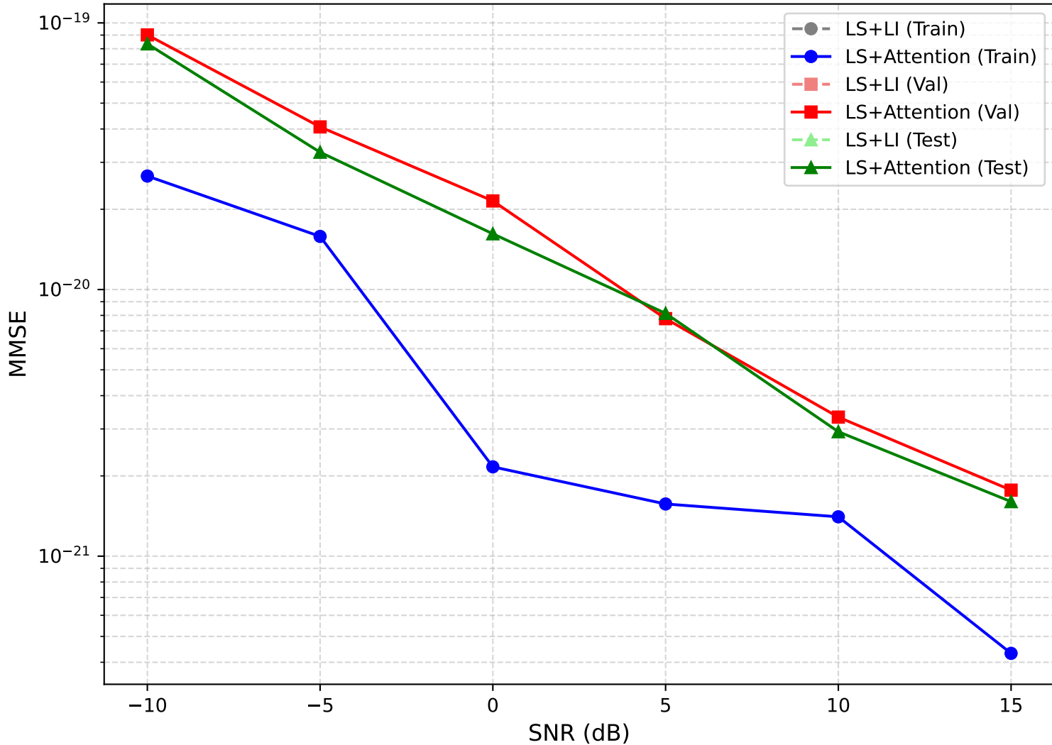
MMSE Comparison over SNR (LS)
