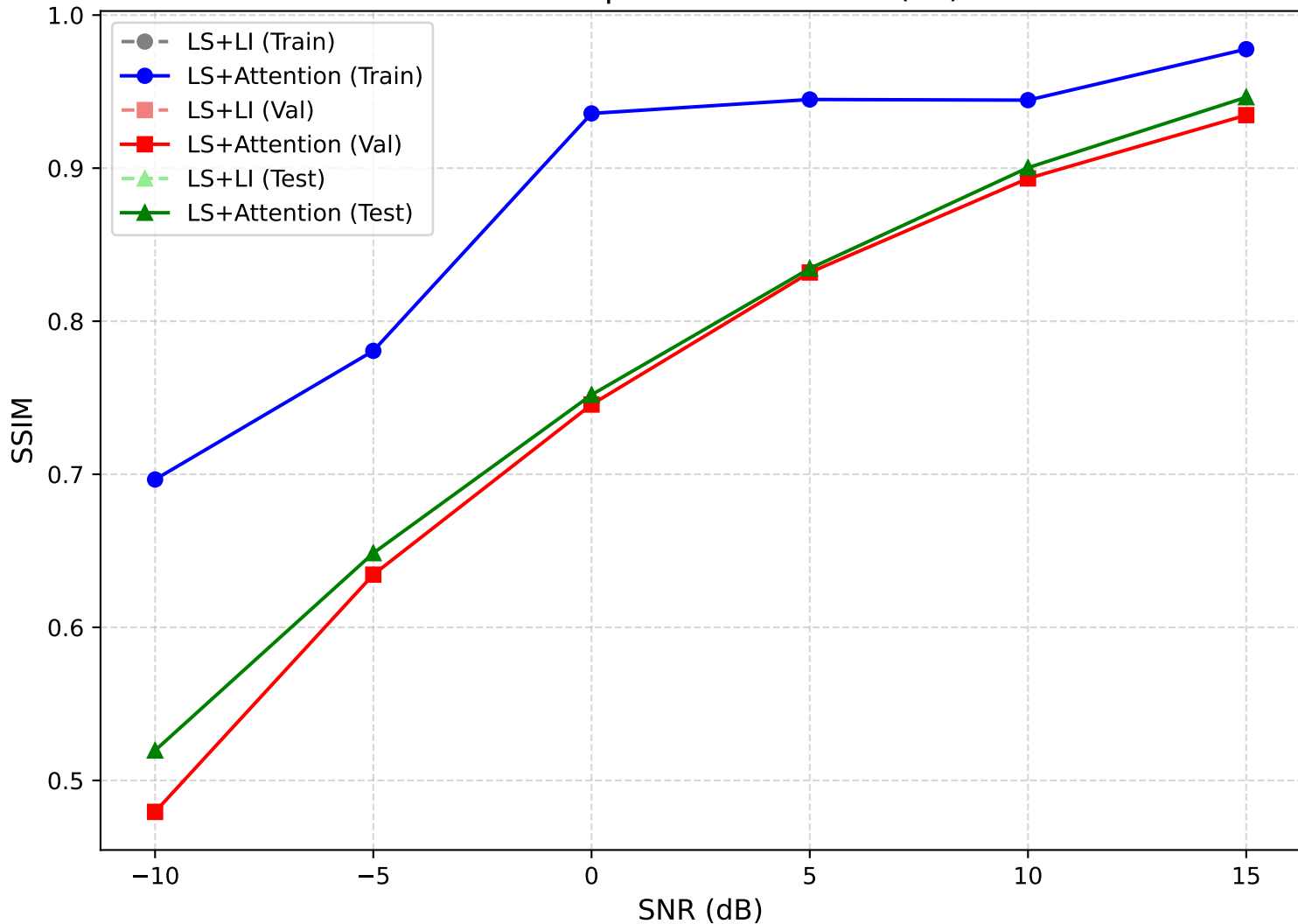
SSIM Comparison over SNR (LS)
