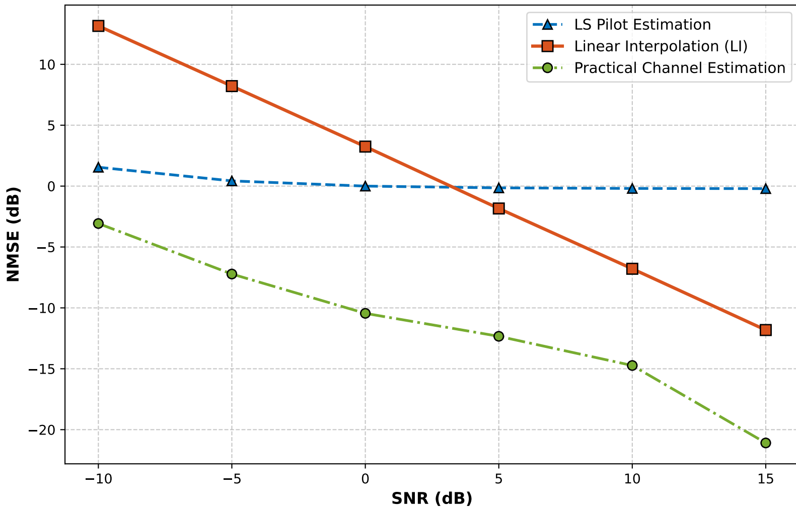
Channel Estimation NMSE Comparison vs. SNR
