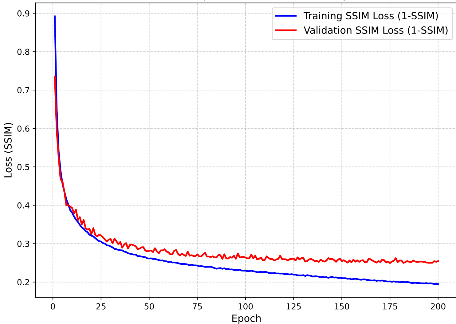
SSIM Loss Component (1 - SSIM) over Epochs
