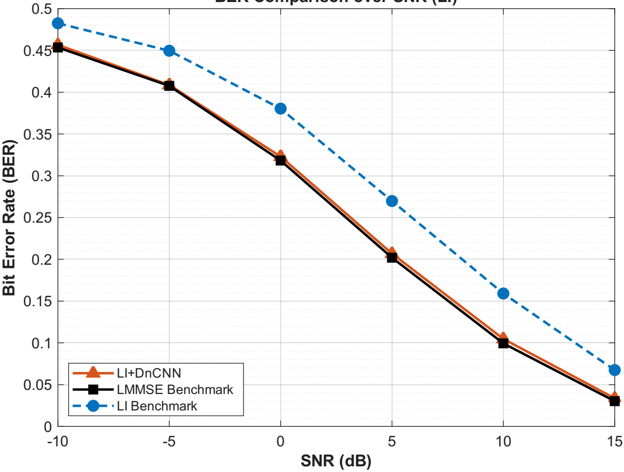
BER Comparison over SNR (LI)
