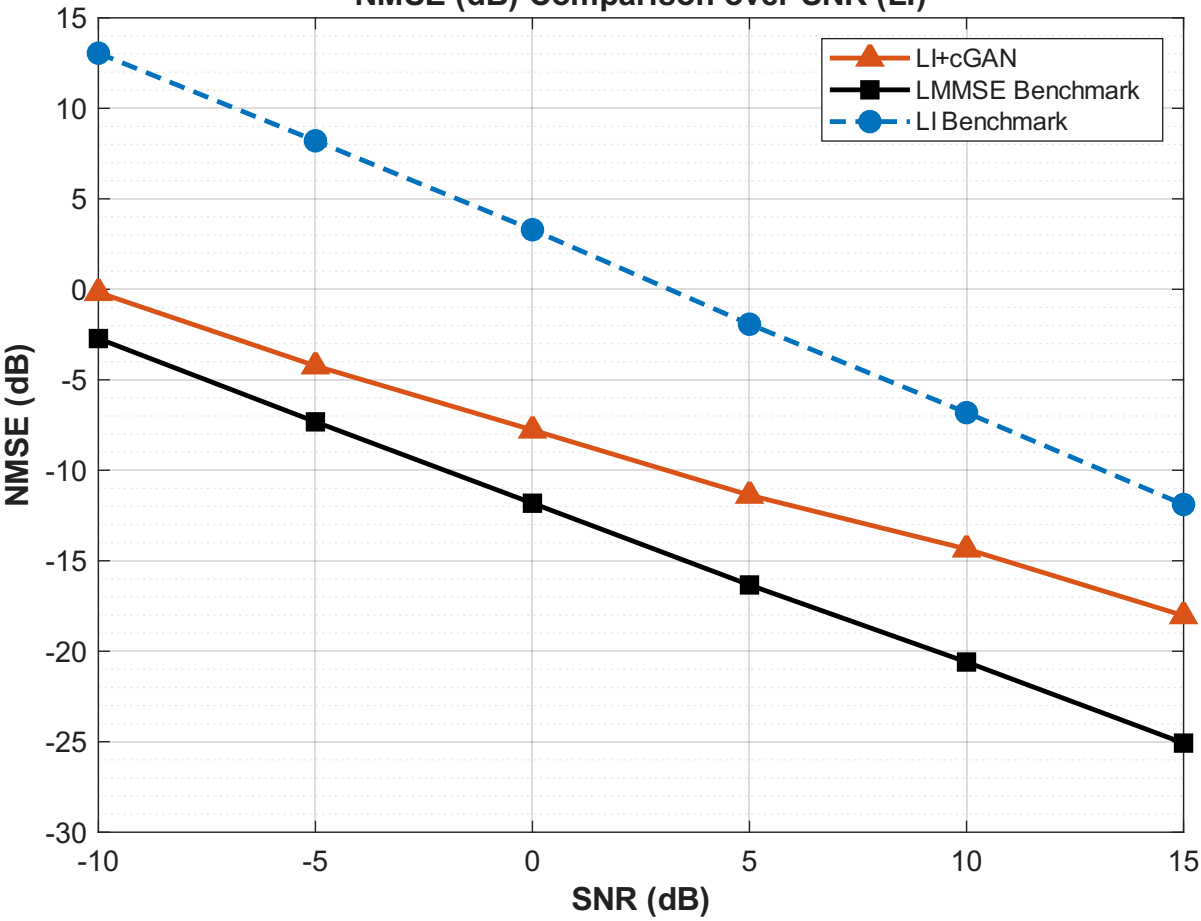
NMSE (dB) Comparison over SNR (LI)
