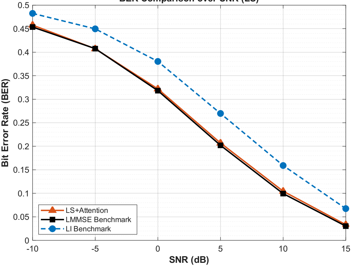
BER Comparison over SNR (LS)
