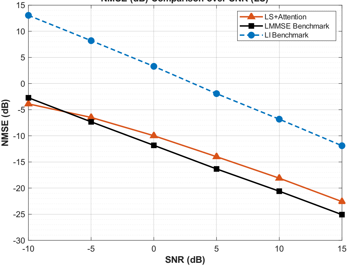
NMSE (dB) Comparison over SNR (LS)
