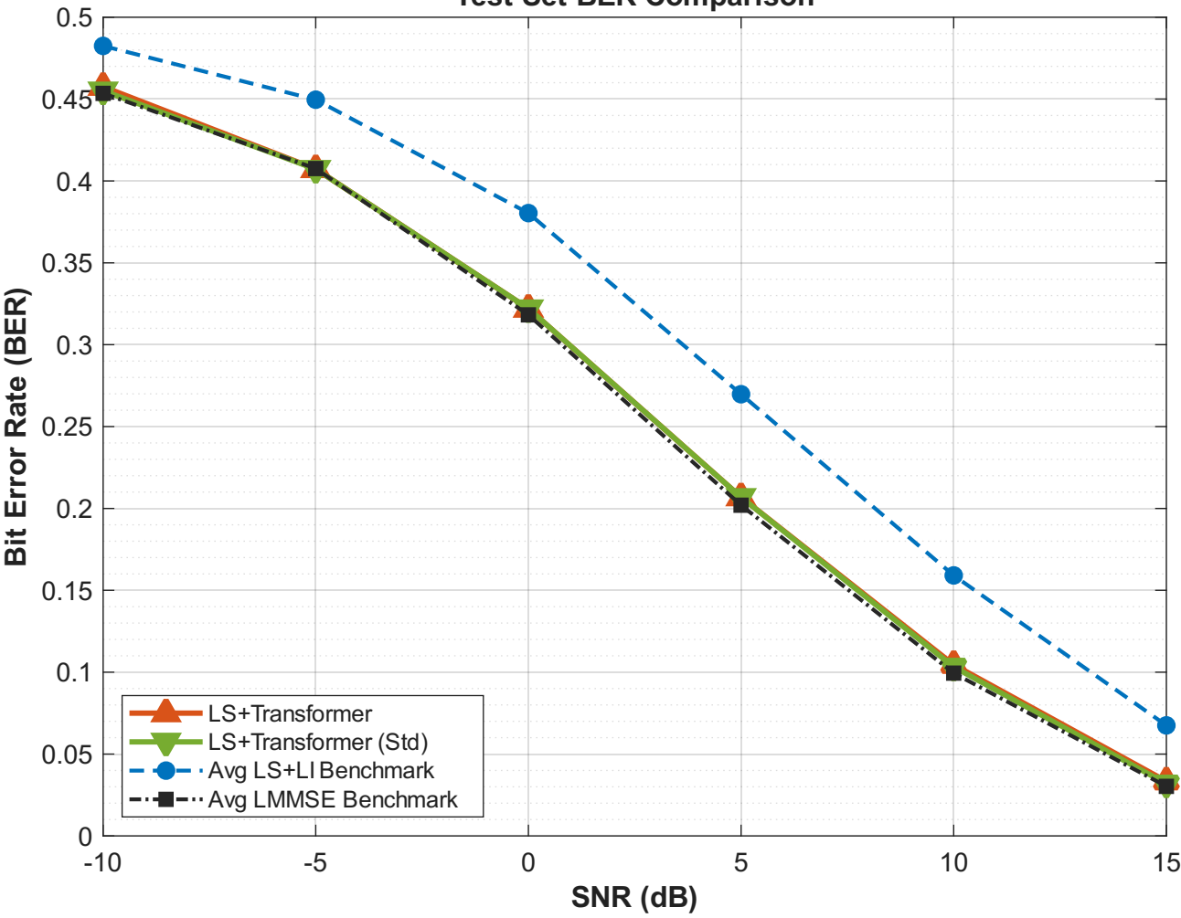
Test Set BER Comparison
