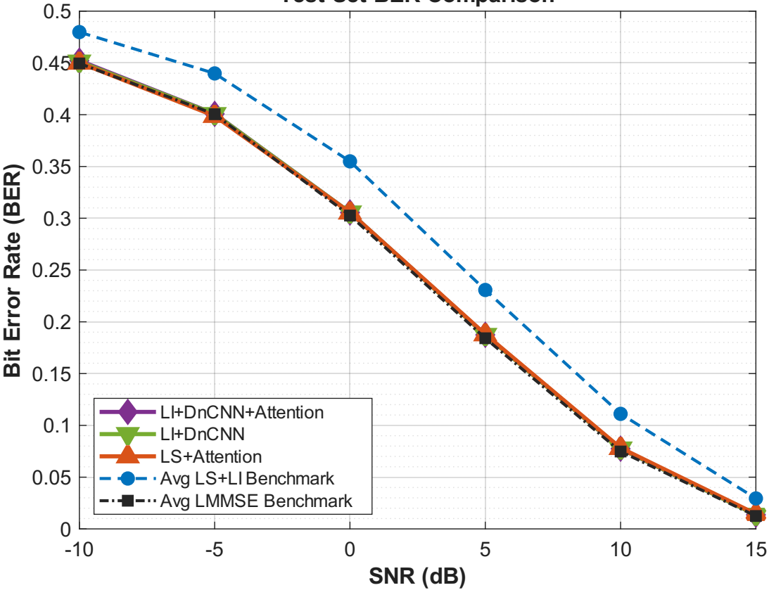
Test Set BER Comparison
