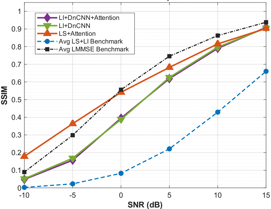
Test Set SSIM Comparison
