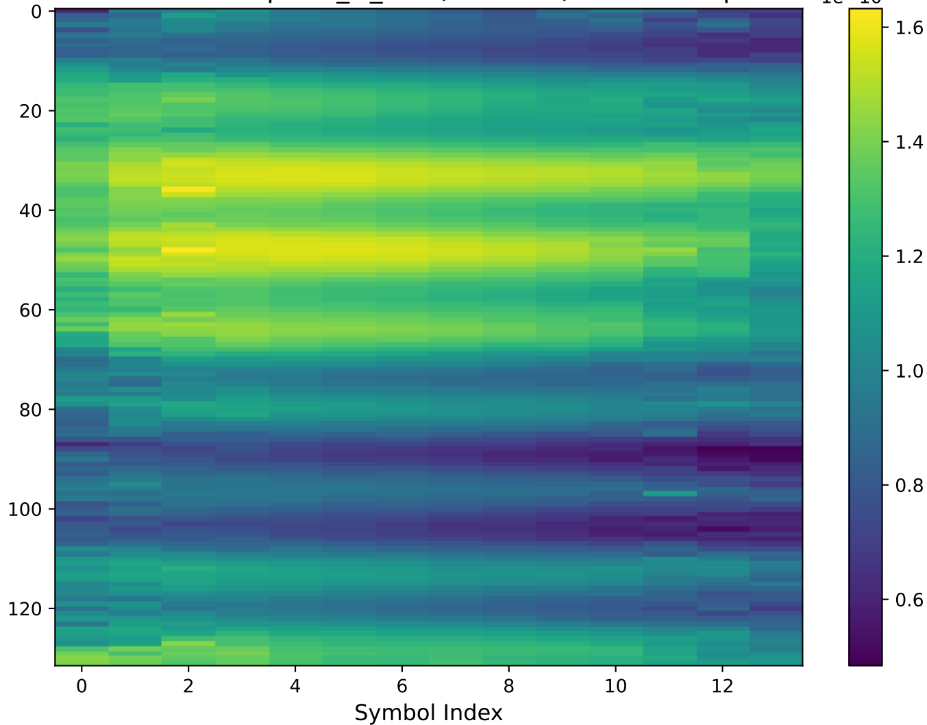
CNN Model Output H_Is_cnn (Real Part) - Train Sample 1
