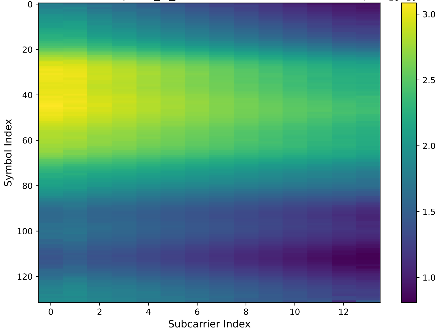
HA02 Model Output H_Is_attention (Real Part) - Train Sample 1_{\text{e}-10}
