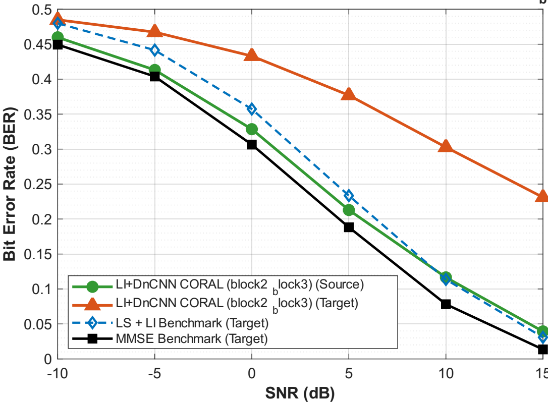
BER: Source vs Target Domain Adaptation (LI+DnCNN CORAL (block2 b lock3))
